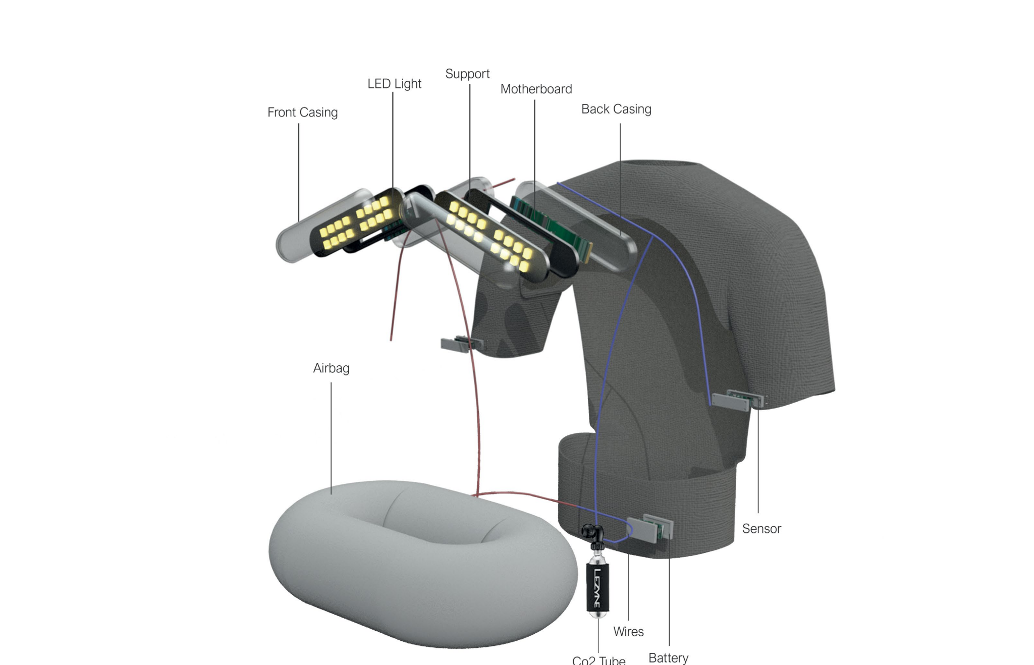
Product Exploded View
